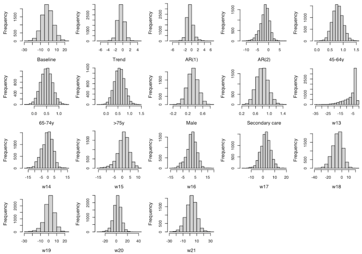
Supplementary Figure 2. State-space model posterior distribution for the key parameters.
