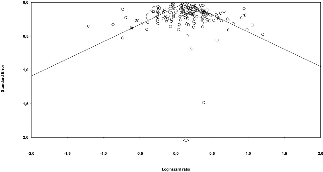
eFigure 4. Funnel Plot for Overall Survival Analysis
