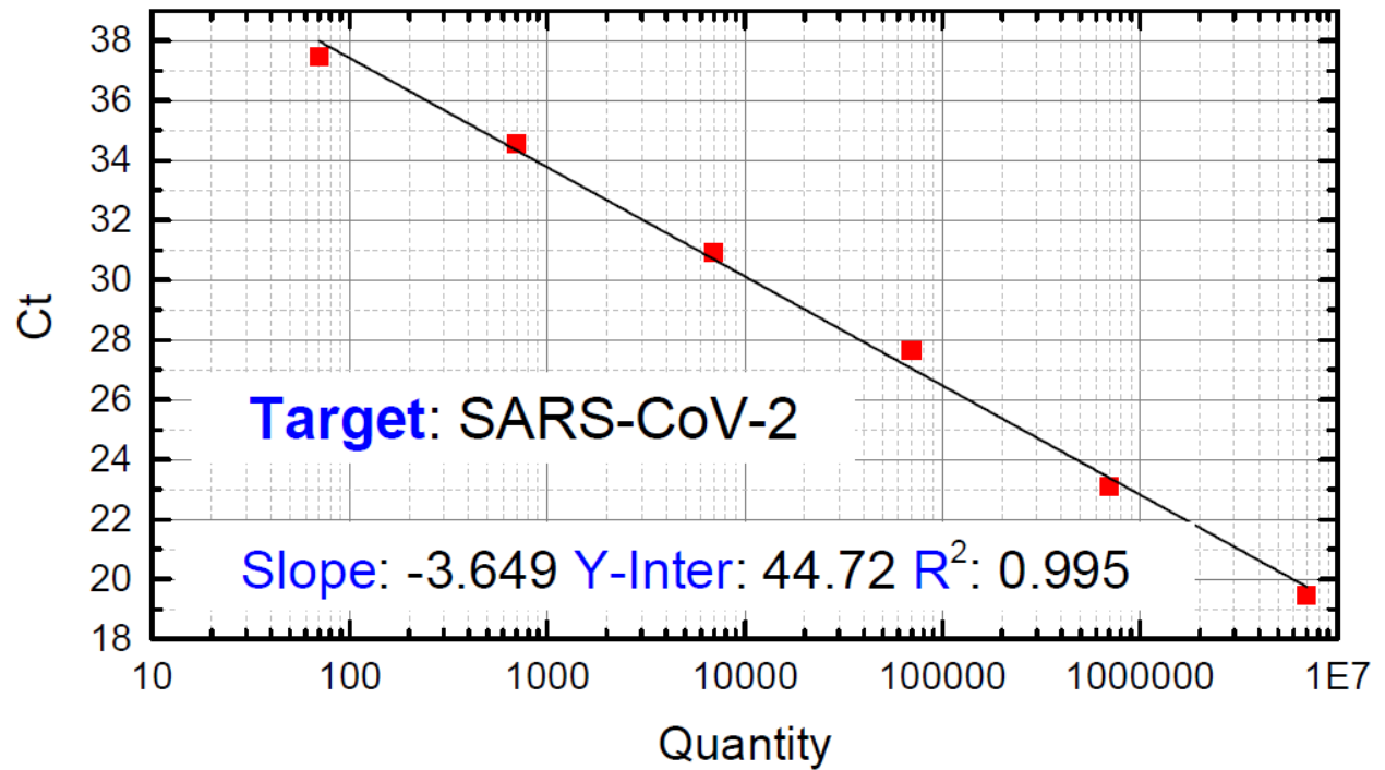
Supplementary Figure 1. Standard curve of the RT-PCR test for three positive SARS-CoV-2 cases.
