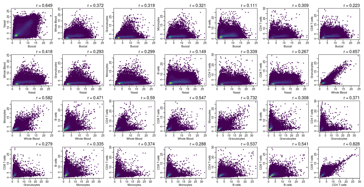
Figure S10. Scatterplot of the site-specific variance in DNA methylation between different sample types across DNAm sites with significantly different levels of variation (n = 194, 247). Above each plot is the Pearson correlation coefficient.
