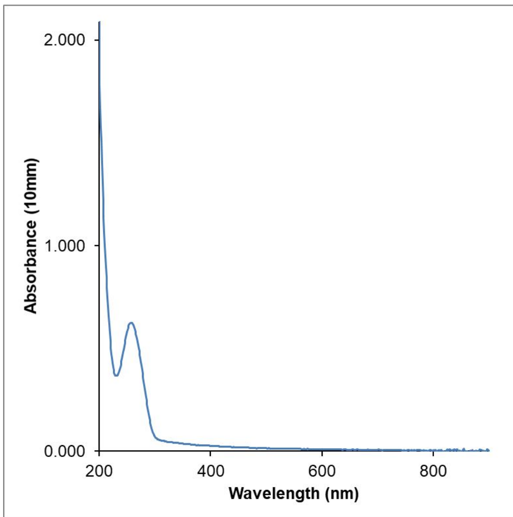
Supplementary Figure S1. The UV spectra of EPS in the range 200-900 nm.
