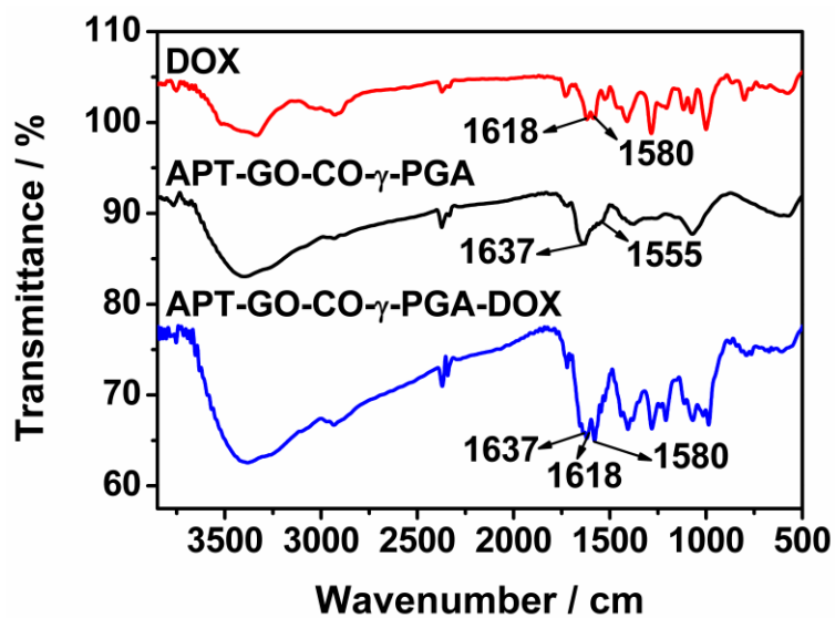
Figure S2. FTIR spectra of DOX, GO-CO- \gamma -PGA-DOX and APT-GO-CO- \gamma -PGA-DOX.
