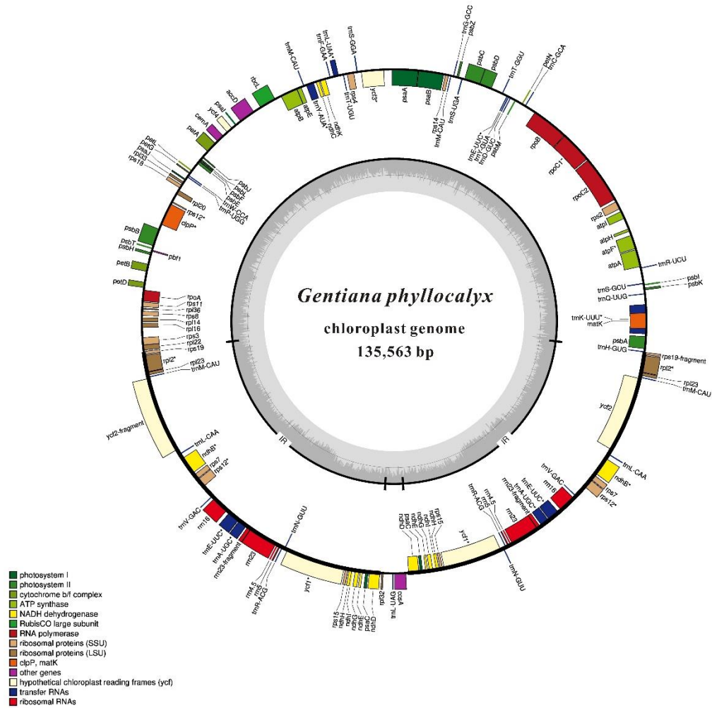
FIGURE B1 Map of the plastome of Gentiana phyllocalyx . Genes drawn inside the circle are transcribed clockwise, and those drawn outside are transcribed counterclockwise. Genes belonging to different functional groups are shown in different colours.
