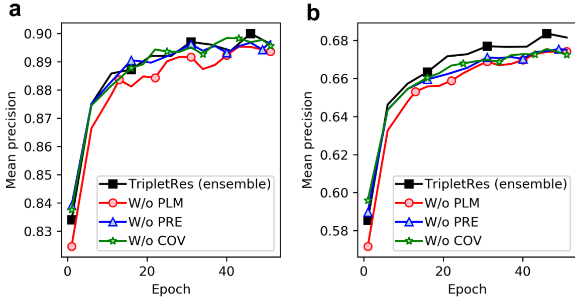
S1 Fig. Comparison of the average precisions over training epochs without individual coevolutionary features and the TripletRes model that ensembles all three sets of features, on the validation set. (a) top- L/5 precision, (b) top- L precision.
