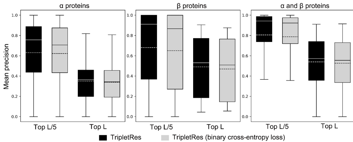
S2 Fig. Comparison of long-range top- L/5 and top- L precisions with different loss functions on the different fold types, where median precision and mean precision are marked in solid and dash lines, respectively.
