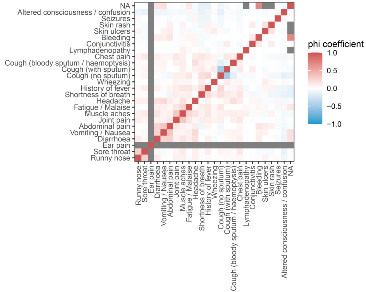
Supplemental Figure 1: Heatmap for correlation between symptoms
