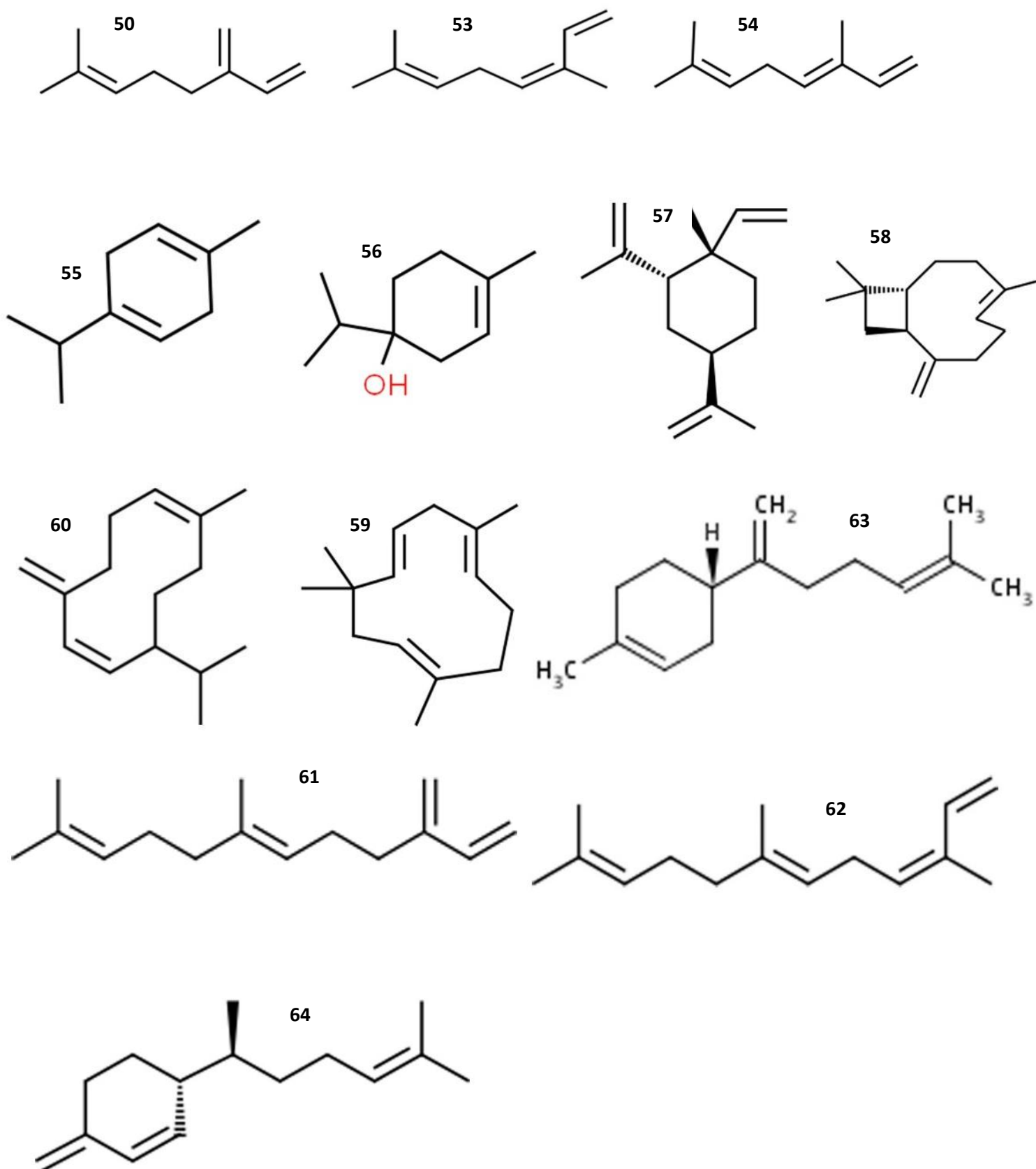
Figure S1: Structure of phytochemicals in S. acmella
