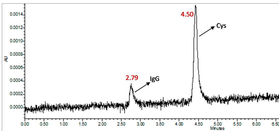
Figure S1: Separation chromatogram of IgG.
