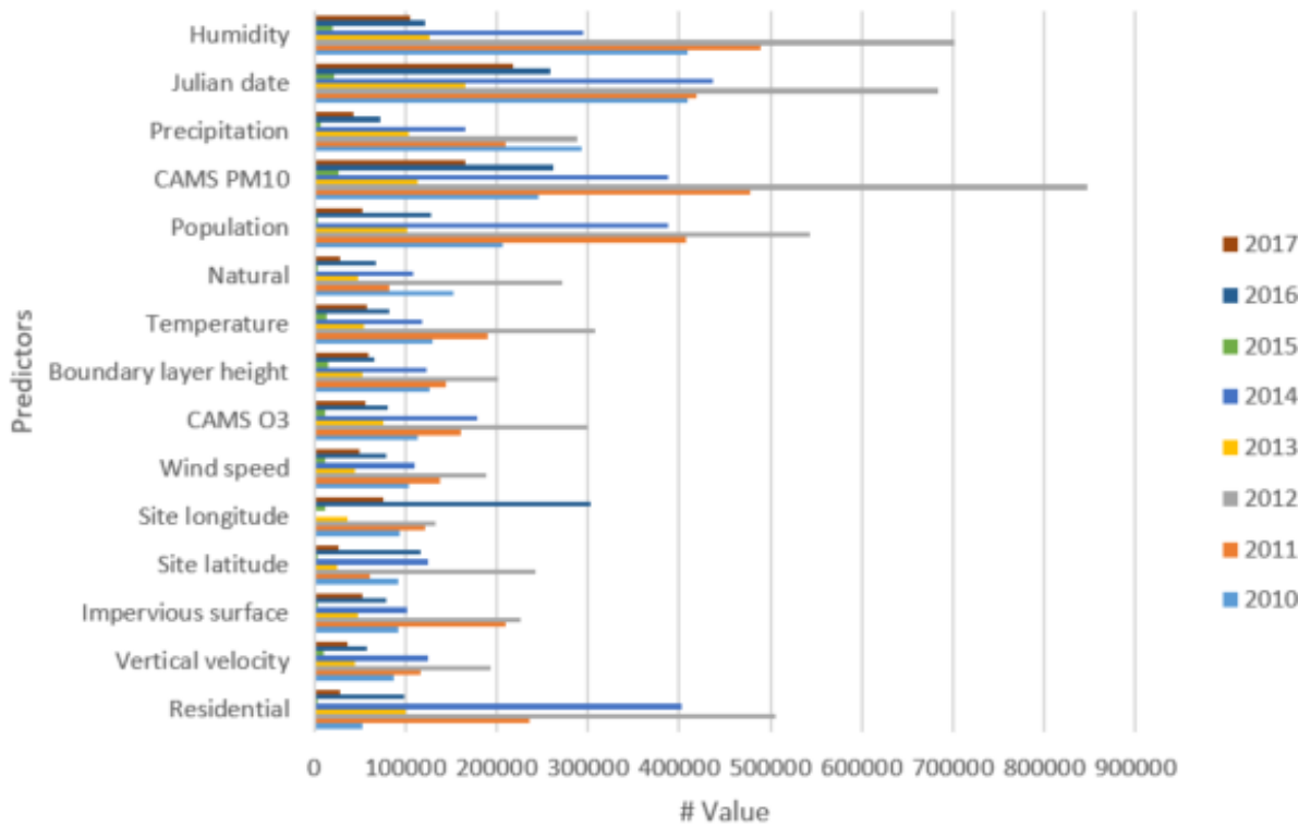
Figure S2: Gauteng province Random Forest Variable of Importance
