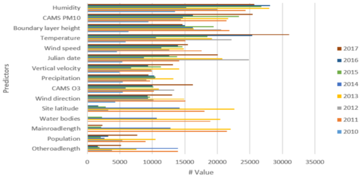
Figure S3: Western Cape province Random Forest Variable of Importance
