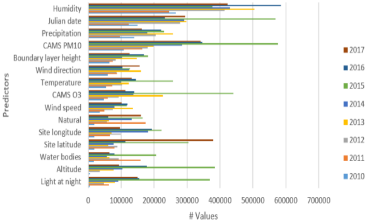
Figure S1: Mpumalanga province Random Forest Variable of Importance
