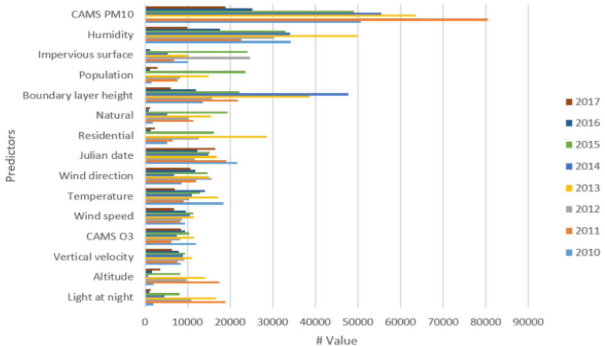
Figure S4: KwaZulu-Natal province Random Forest Variable of Importance
