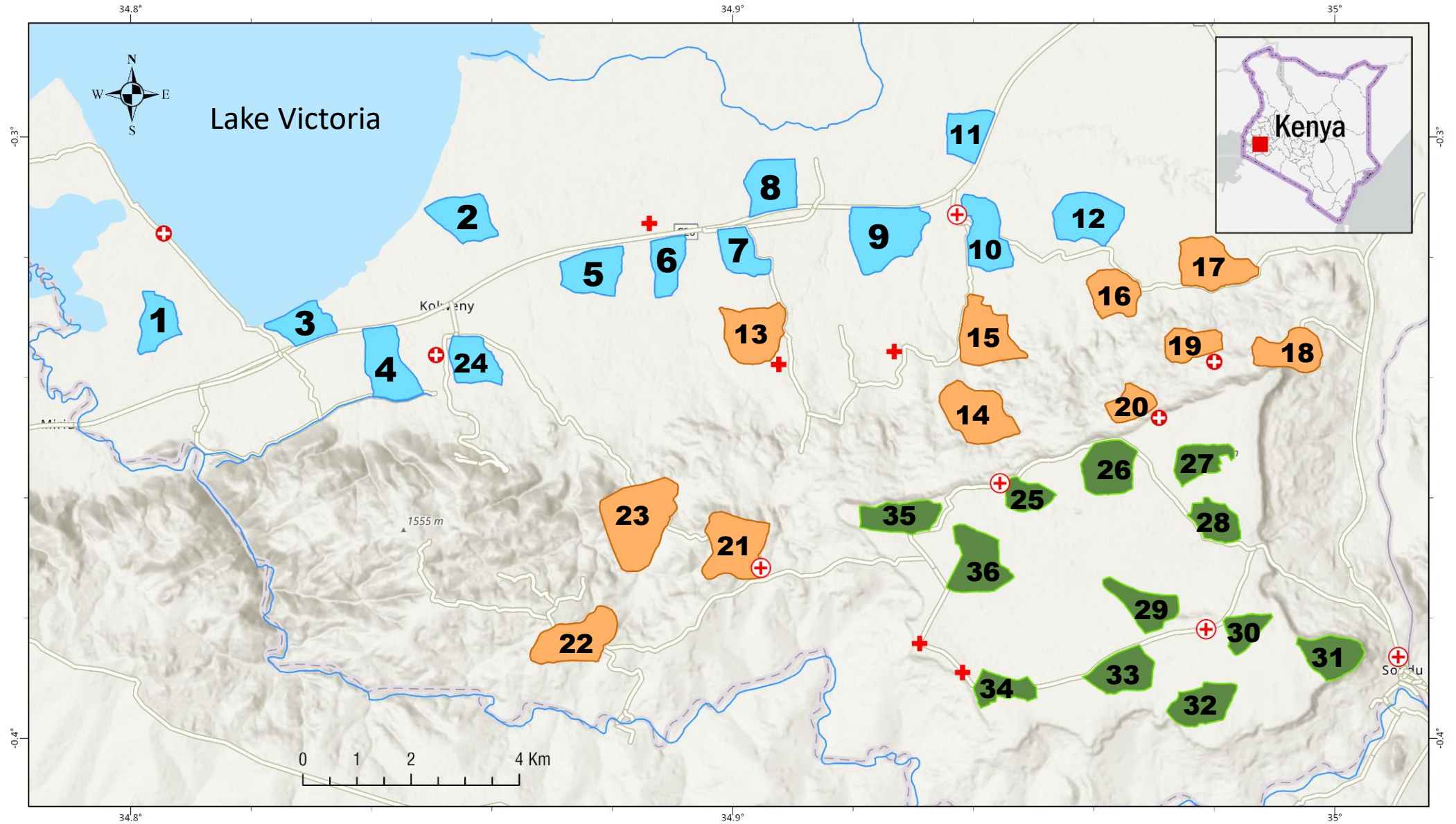
Supplementary Figure S1. Distribution of clusters/villages after adjusted for altitude. Numbers represented village labels used in Figure 5. This is a simplified version of Figure 6 without showing locations of habitats.
