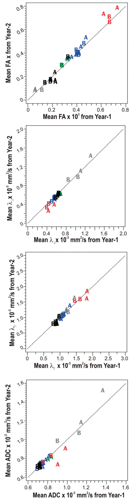
On-line Fig 2. Correlation of longitudinal DTI measures within the same magnet across a major system upgrade (Siemens TIM upgrade; year 0 versus years 1 and 2) and after the upgrade (year 1 versus year 2). Red indicates the corpus callosum; blue, deep white matter; green, subcortical white matter; gray, cortical gray matter; black, deep gray matter. A and B represent the 2 healthy volunteers who were imaged in the study.
