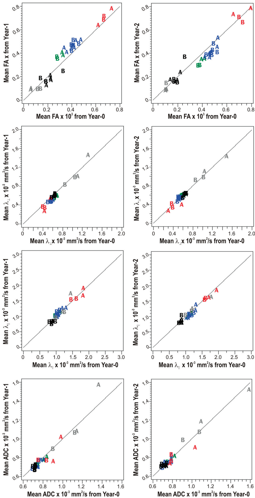
On-line Fig 2. Correlation of longitudinal DTI measures within the same magnet across a major system upgrade (Siemens TIM upgrade; year 0 versus years 1 and 2) and after the upgrade (year 1 versus year 2). Red indicates the corpus callosum; blue, deep white matter; green, subcortical white matter; gray, cortical gray matter; black, deep gray matter. A and B represent the 2 healthy volunteers who were imaged in the study.
