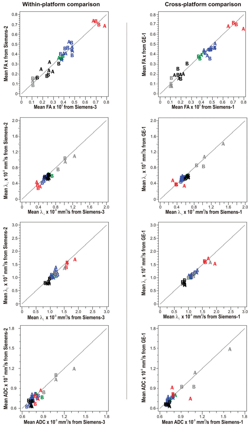
On-line Fig 1. A sample illustration of the concordance plots of DTI measures across different magnets and imaging platforms. Red indicates the corpus callosum; blue, deep white matter; green, subcortical white matter; gray, cortical gray matter; black, deep gray matter. A and B in the graphs represent the 2 healthy volunteers who were imaged in the study.
