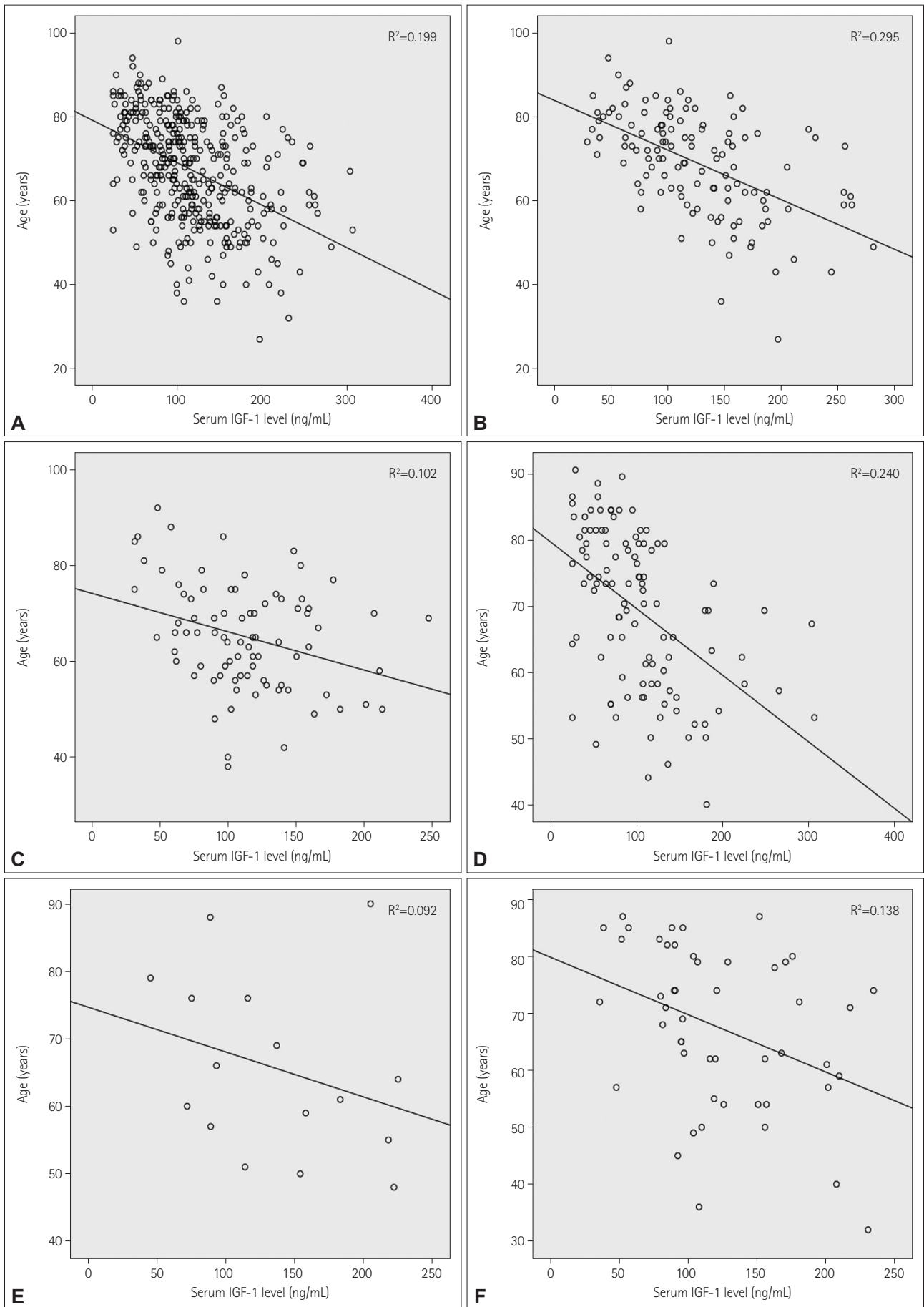
Supplementary Fig. 1. Correlation between serum IGF-1 level and age according to stroke subtype: all patients (A), and in patients with large-artery atherosclerosis (B), small-vessel occlusion (C), cardioembolism (D), stroke of other determined etiology (E), and stroke of undetermined etiology (F). IGF-1: insulin-like growth factor-1.
