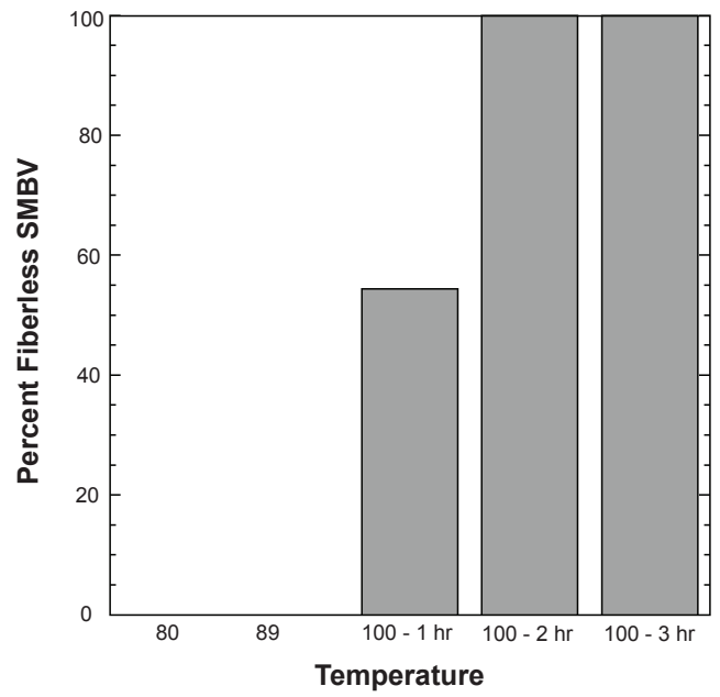
Percent Fiberless Particles vs. Temperature
