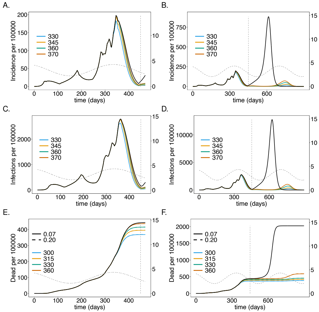
S2 Fig. Onset of the vaccination campaign: As in Fig 4 but for U.S. instead of Germany. Parameters for contact reduction are given in S7 Table.
