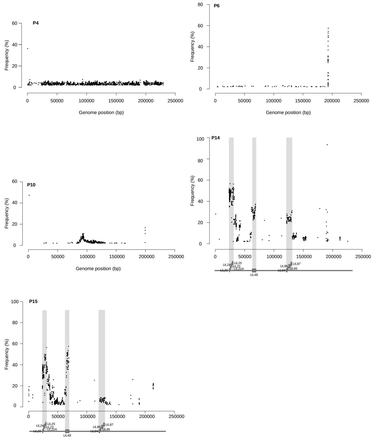
Supplementary Figure 3. Distribution of heterozygous variants. The genomic location and frequency of heterozygous variants is shown for all isolates. For P14 and P15, a schematic representation of the HCMV genome is shown at the bottom to visualize the regions where most high-frequency variants occur (shaded areas).
