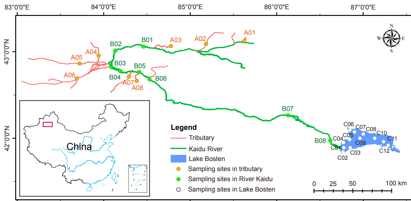
Figure S1. Overview map of the River Kaidu catchment showing the sampling sites in upstream tributaries (A01~A08), River Kaidu (B01~B08) and Lake Bosten (C01~C12).
