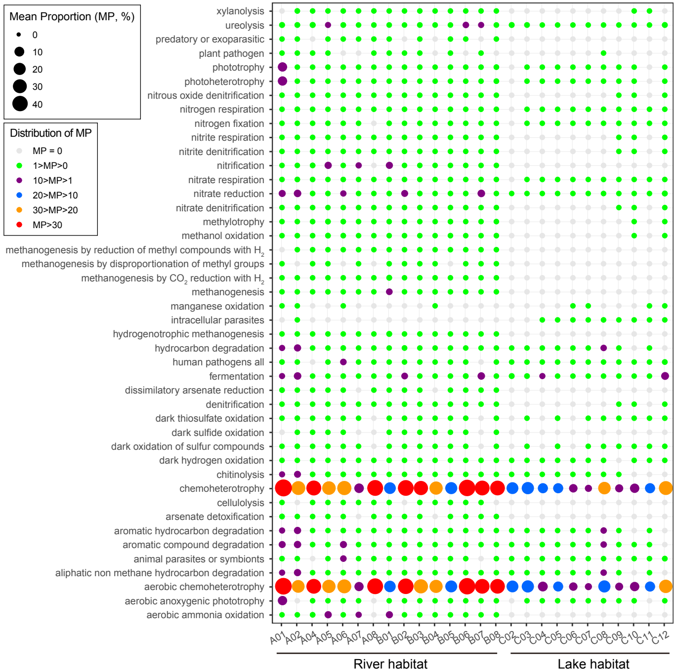
Figure S5. Mean proportions of predicted functional groups across samples from river habitats (upstream tributaries and mainstream of the Kaidu River, n = 15 ) to lake habitats (Lake Bosten, n = 11 ).
