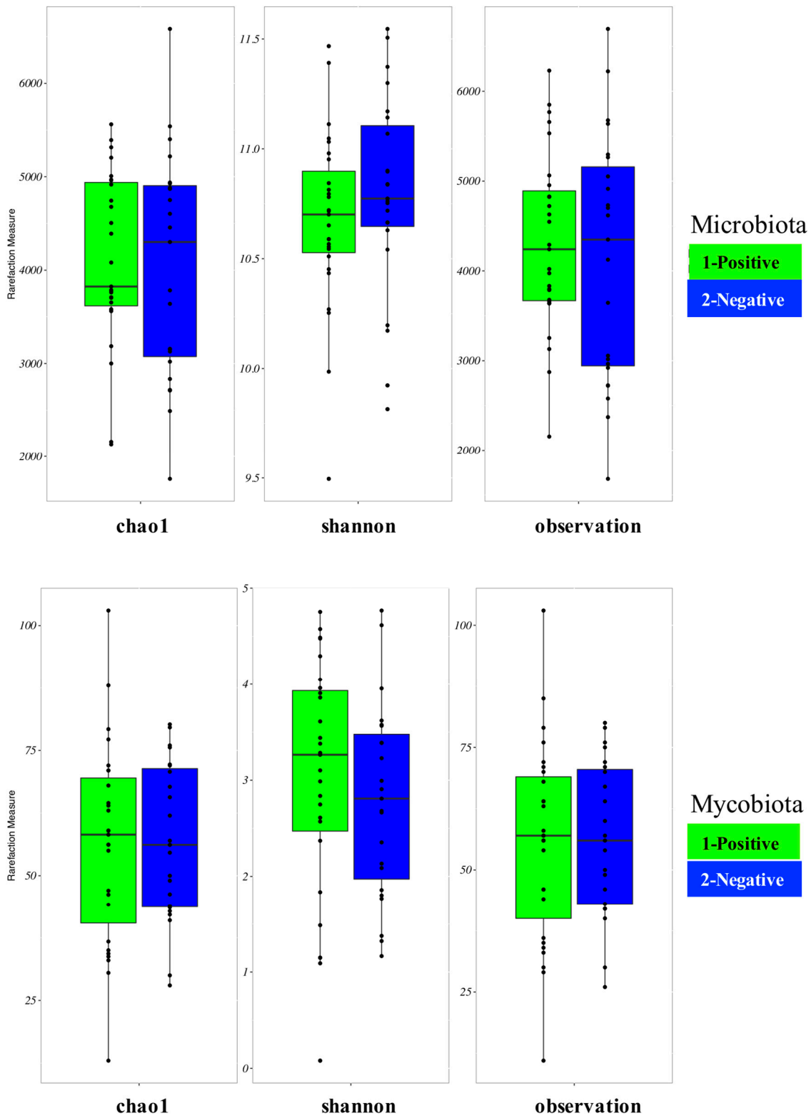
Figure Supplementary 1. Microbiota and mycobiota \alpha -diversity by response to the DBPC gluten challenge test
