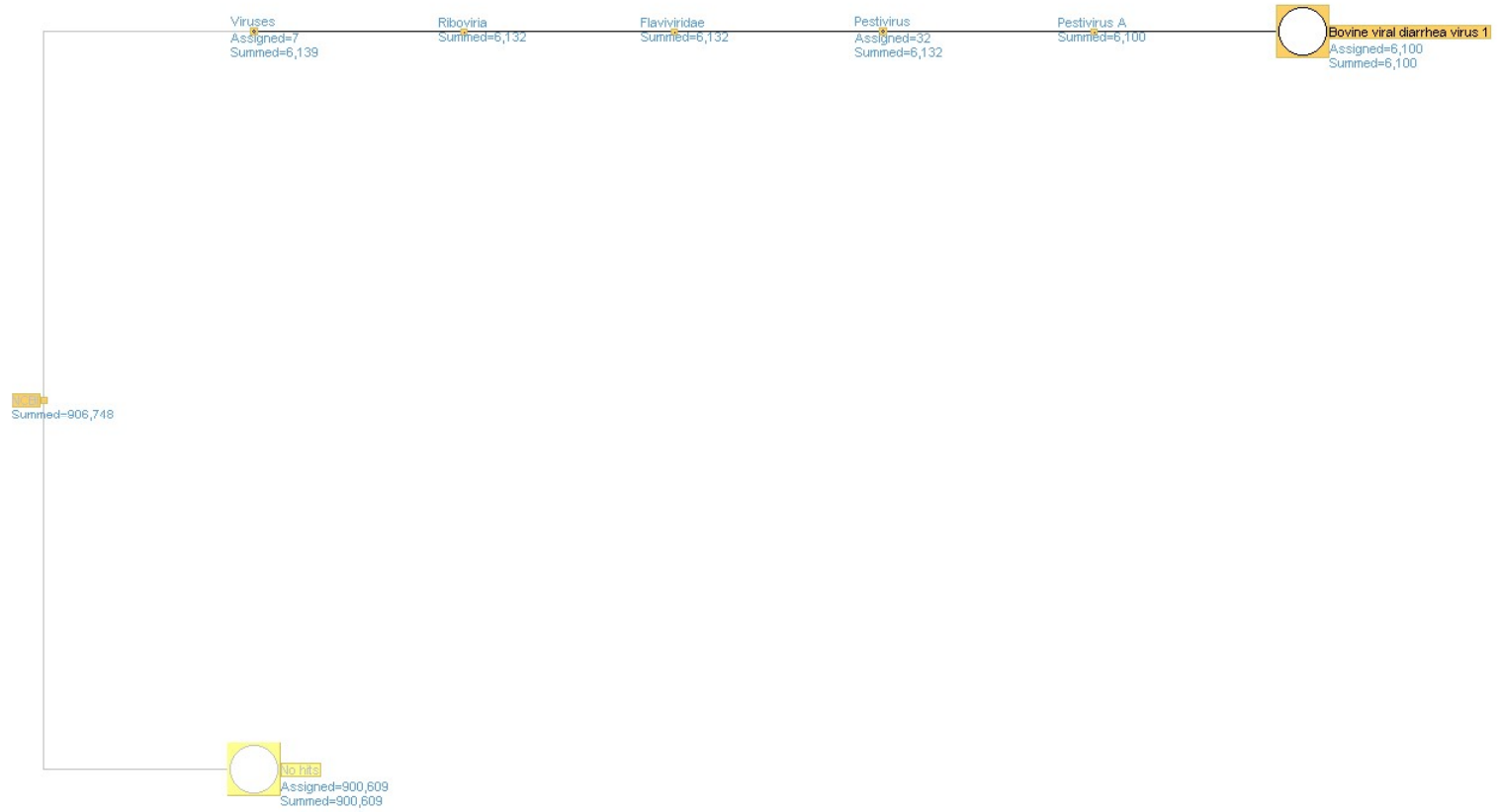
Figure 1: Top hits against known bovine virus sequences for S_33
