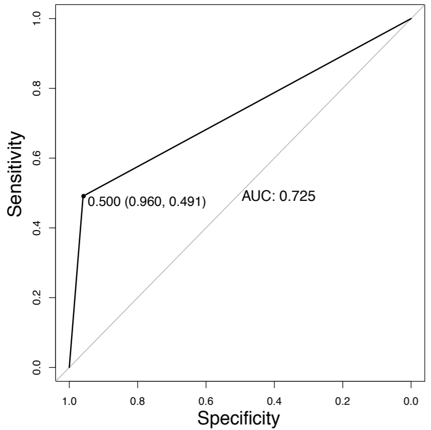
CK-MB
