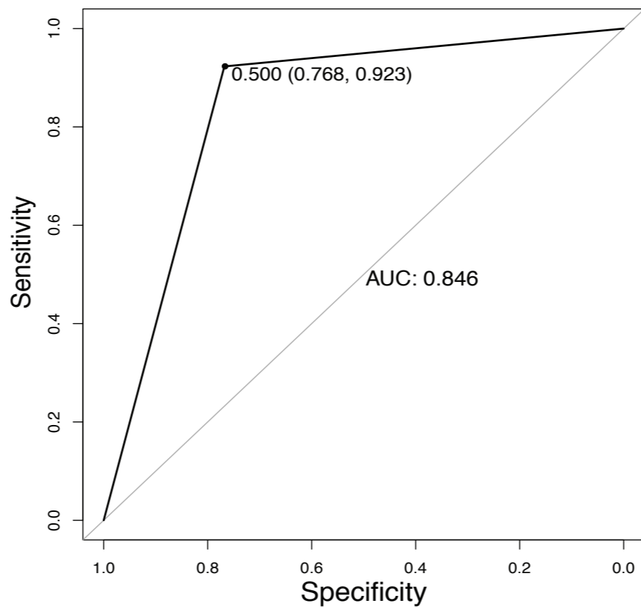
LDH
