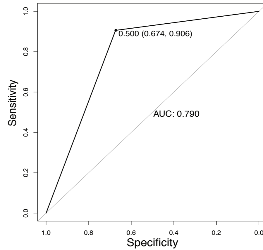
\alpha -HBDH
