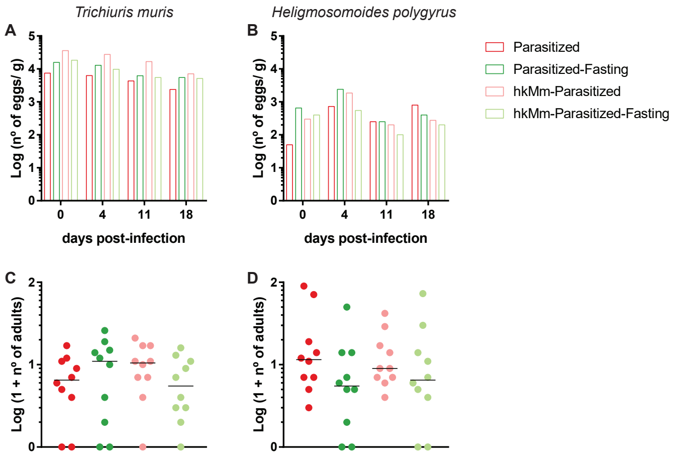
Supplementary figure 3: Recount of helminth eggs in faeces during the experiment (A-B, bars represent means of 2 cages) and adult parasites in intestines at final endpoint (C-D, each circle represents an animal and lines are medians). A and C correspond to T. muris and B and D are H. polygyrus .
