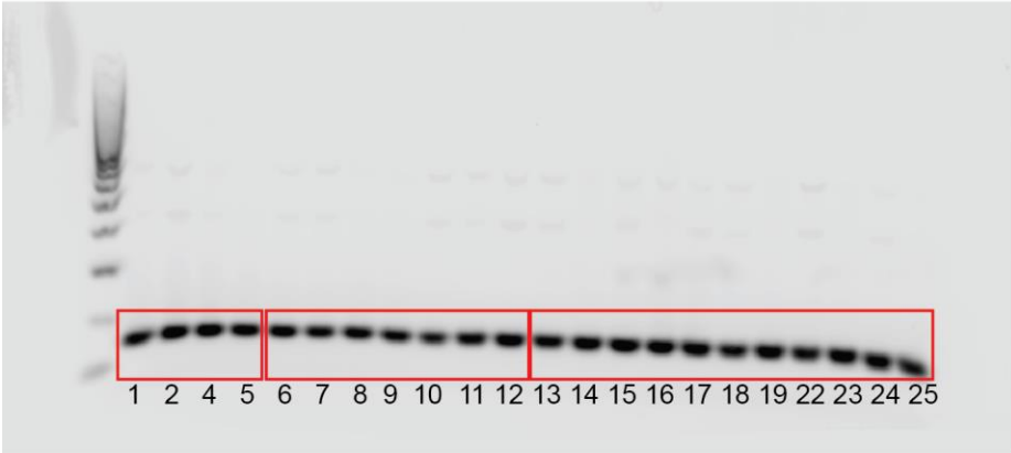
Actin
