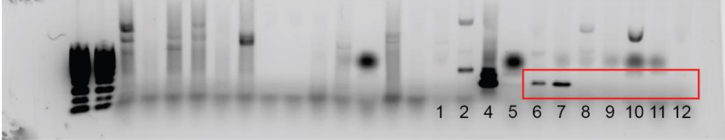
FYN-TRAF3IP2, short exposure
