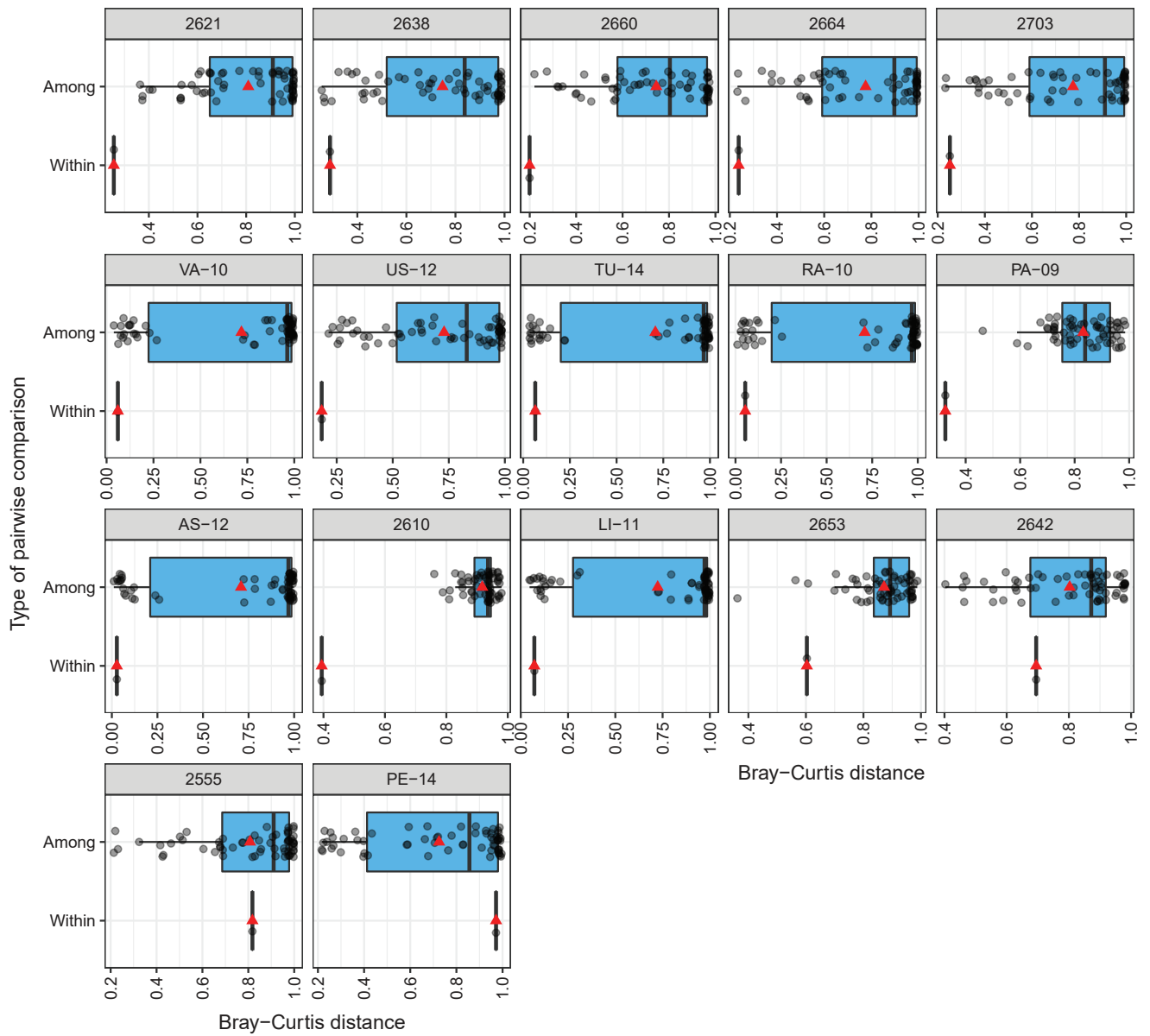
Figure S4. Pairwise distances among samples (MAG data). Horizontal solid lines show medians, red triangles show means.
