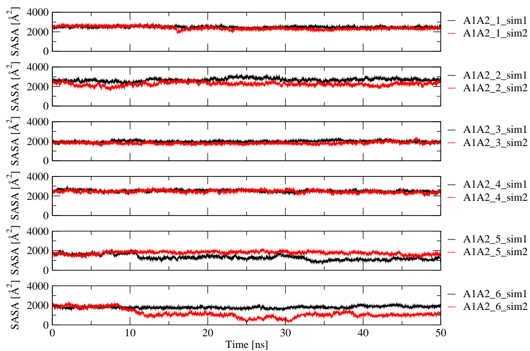
Figure S2: Time series of the SASA buried at the inter-domain interface along the simulations with the A1A2 complex models.
