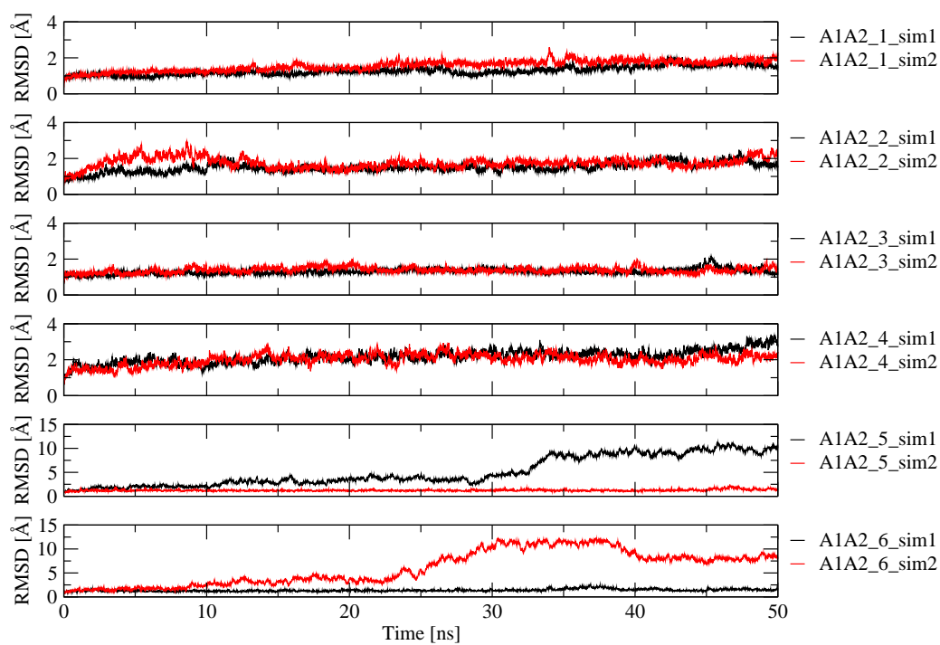
Figure S1: Time series of the C_{\alpha} RMSD from the initial conformation along the simulations with the A1A2 complex models.
