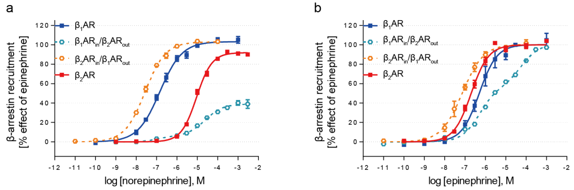
Supplementary information, Fig. S3 | \beta_1 AR, \beta_2 AR and \beta_1 AR in / \beta_2 AR out , \beta_2 AR in / \beta_1 AR out chimeras.
