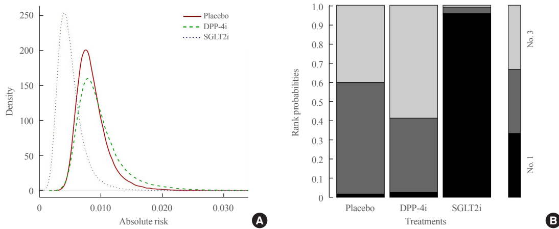
Supplemental Fig. S6. Sensitivity analysis of end-stage kidney disease by excluding Perkovic, 2019 (CREDESCENCE) study. (A) Absolute risks and (B) rank probabilities of the treatments. CREDESCENCE, Canagliflozin and Renal Events in Diabetes with Established Nephropathy Clinical Evaluation; DPP-4i, dipeptidyl peptidase-4 inhibitor; SGLT2i, sodium-glucose cotransporter 2 inhibitor.
