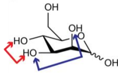
D-Mannopyranose
