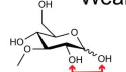
\beta -3-O-methyl-Glucopyranose
