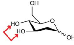
2-deoxy-D-Glucopyranose
