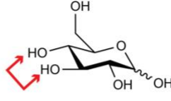
D-Glucopyranose
