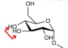
Methyl- \alpha -D-Glucopyranose
