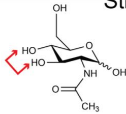
N-acetyl-Glucosamine
