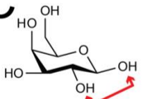
\beta -D-Galactopyranose
