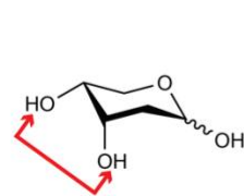
2-deoxy-D-Ribose
