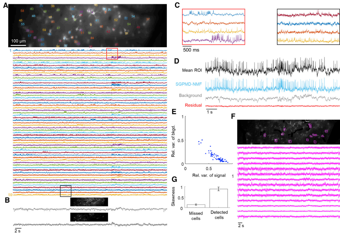
Figure 6. Voltage imaging in mouse cortex L1 using Voltron
