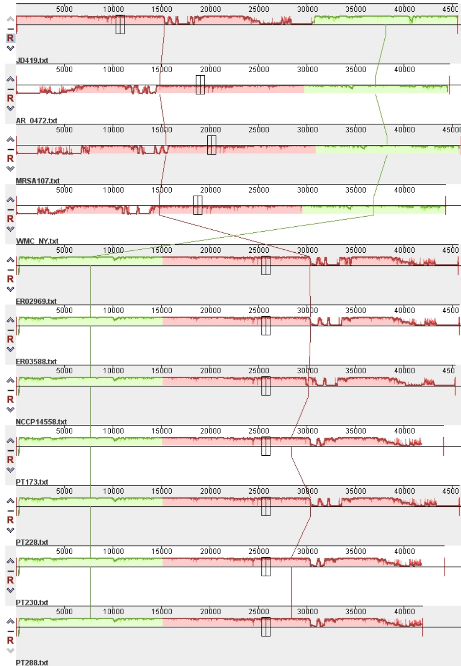
Suppl.Fig.2. Comparative genomic analysis of Staphylococcus phage JD419 with prophages predicted in the corresponding S.aureus strain. (Accession No. MRSA107: CP018629.1; PT288: CP049388.1; AR_0472: CP029649.1; PT228: CP049486.1; ER02969: CP030658.1; ER03588: CP030595.1; NCCP14558: CP013953.1; PT173: CP049580.1; PT230: CP049482.1; WMC_NY: CP063990.1).
