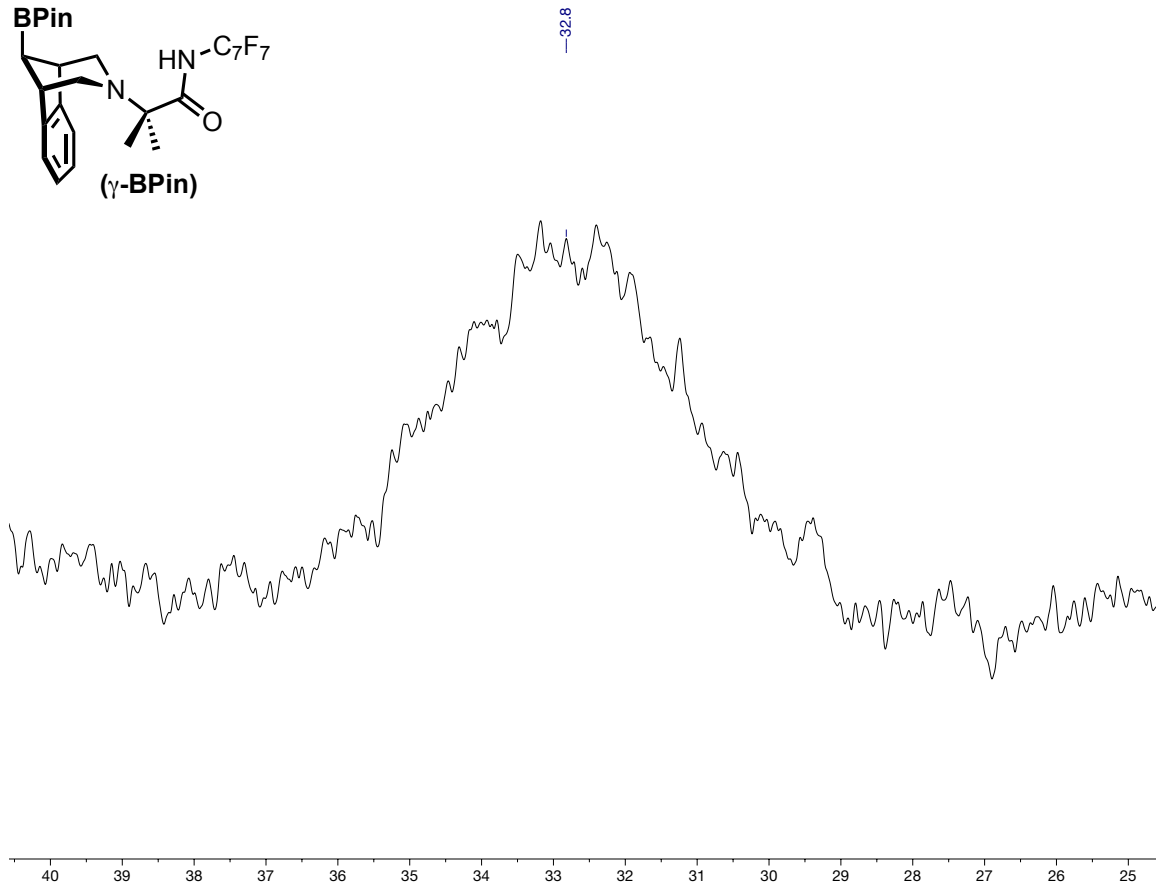
^{11}\text{B} NMR Spectrum in \text{CDCl}_3
