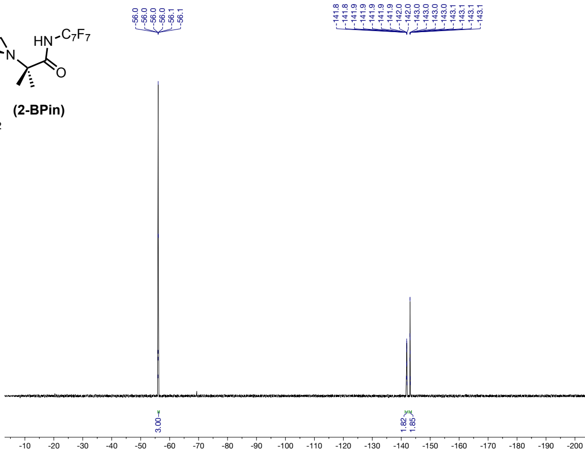
^{19}\text{F} NMR Spectrum in \text{CDCl}_3
