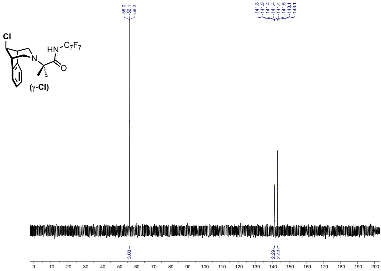
^{19}\text{F} NMR Spectrum in \text{CDCl}_3
