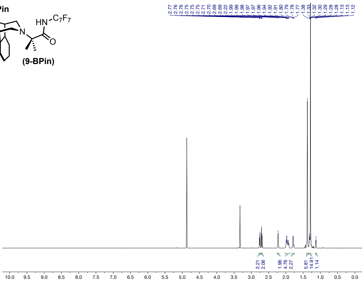
^1\text{H} NMR Spectrum in \text{CD}_3\text{OD}
