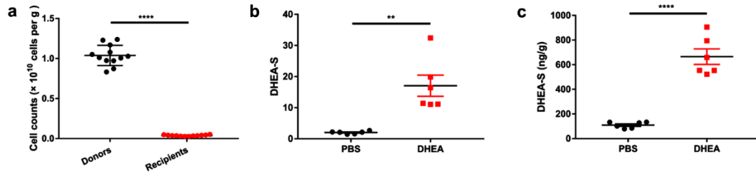
Figure S3. Transplant contents in FMT donors and gut circumstances in antibiotic-treated recipients before FMT initiation.
