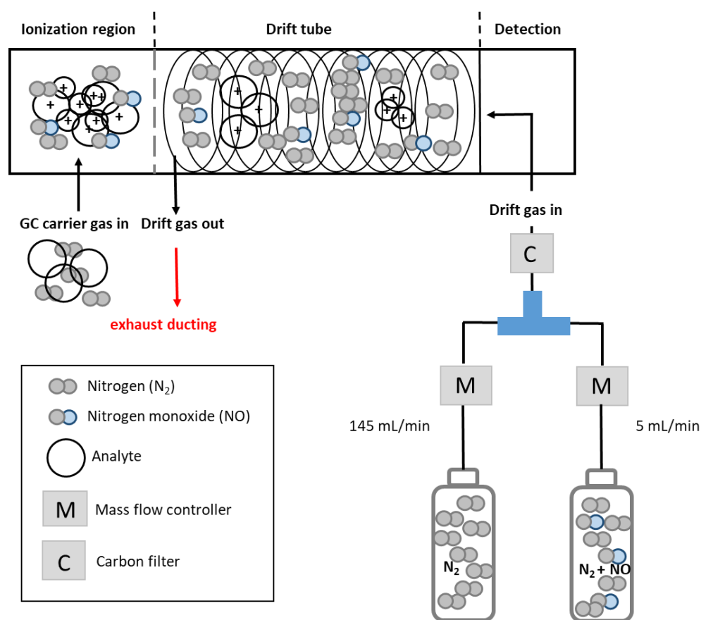
Figure S1 Schematic illustration of the instrument setup.
