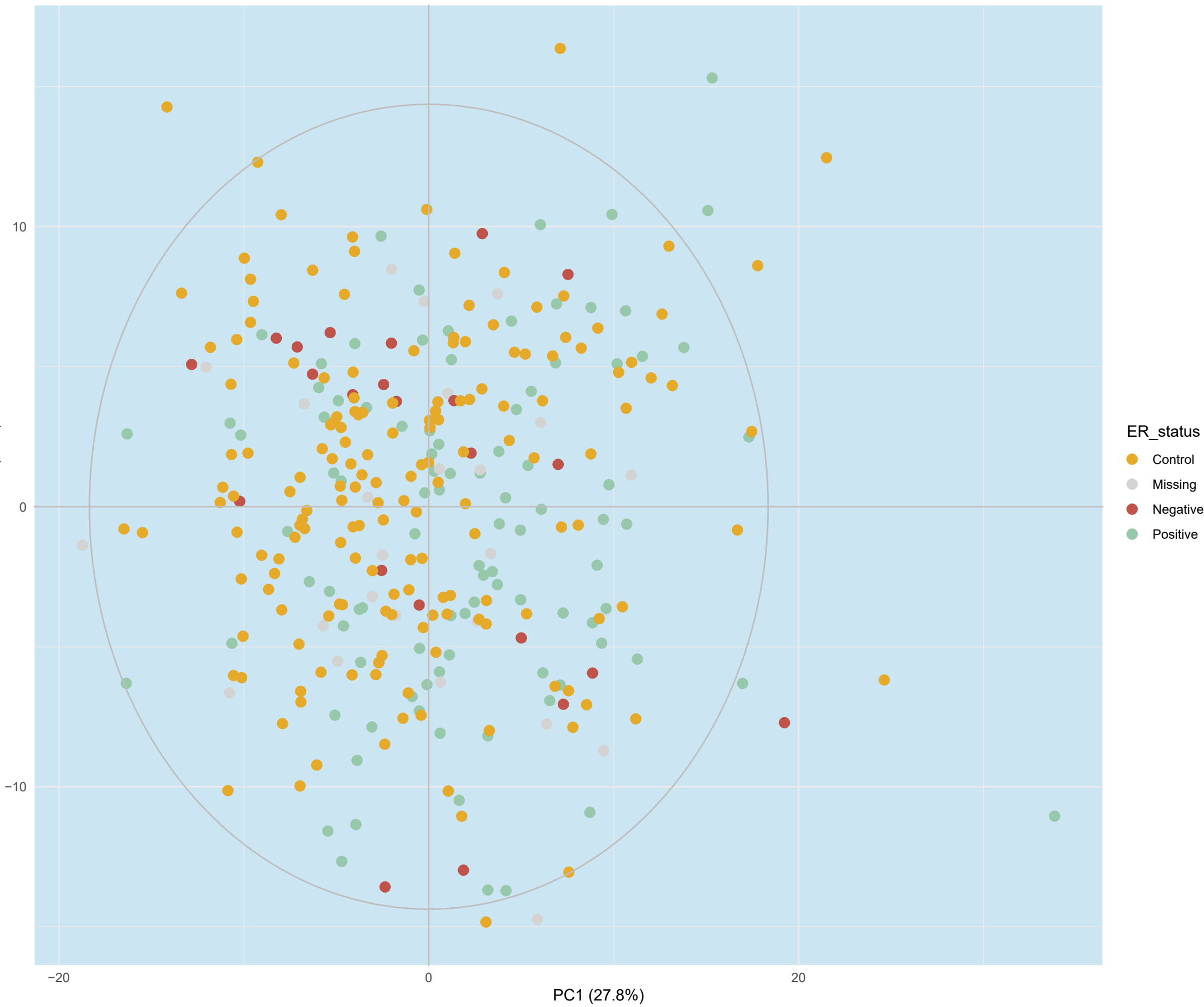
Scores plot
