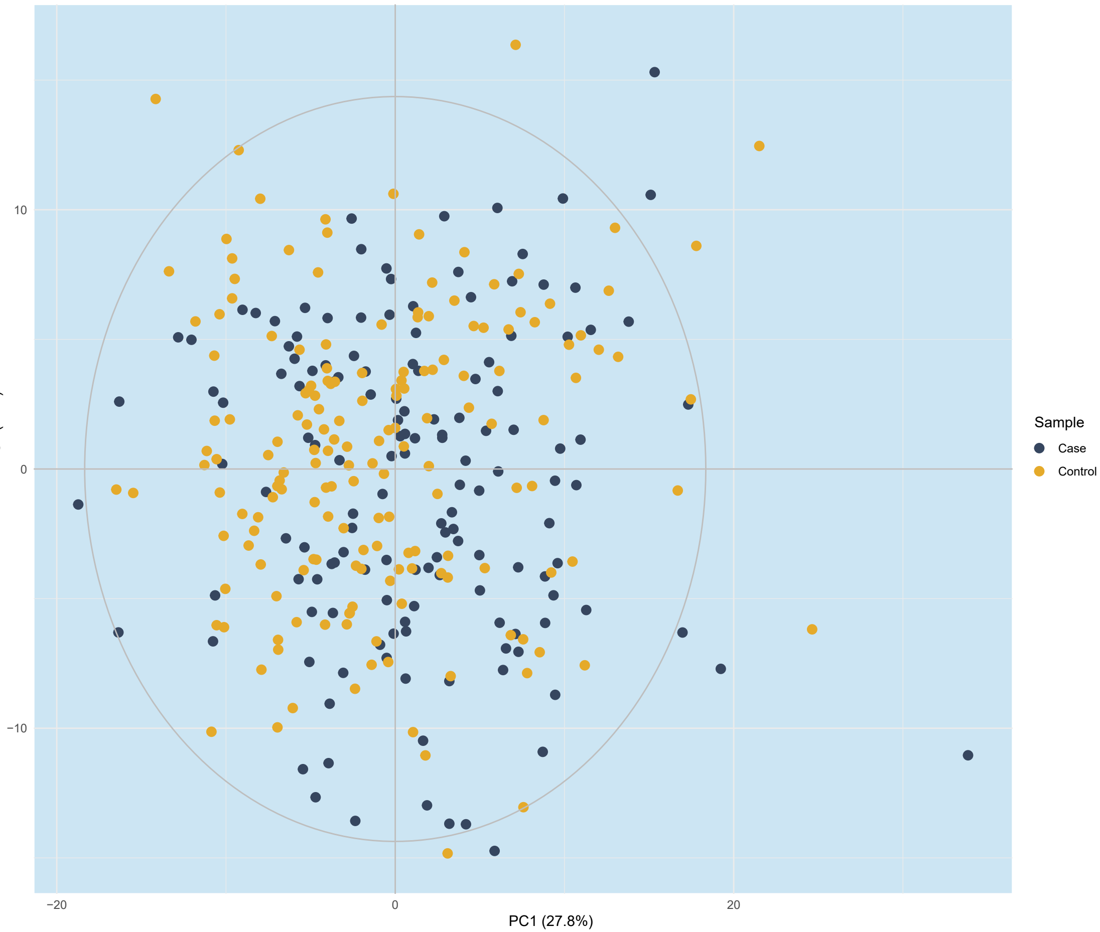
Scores plot
