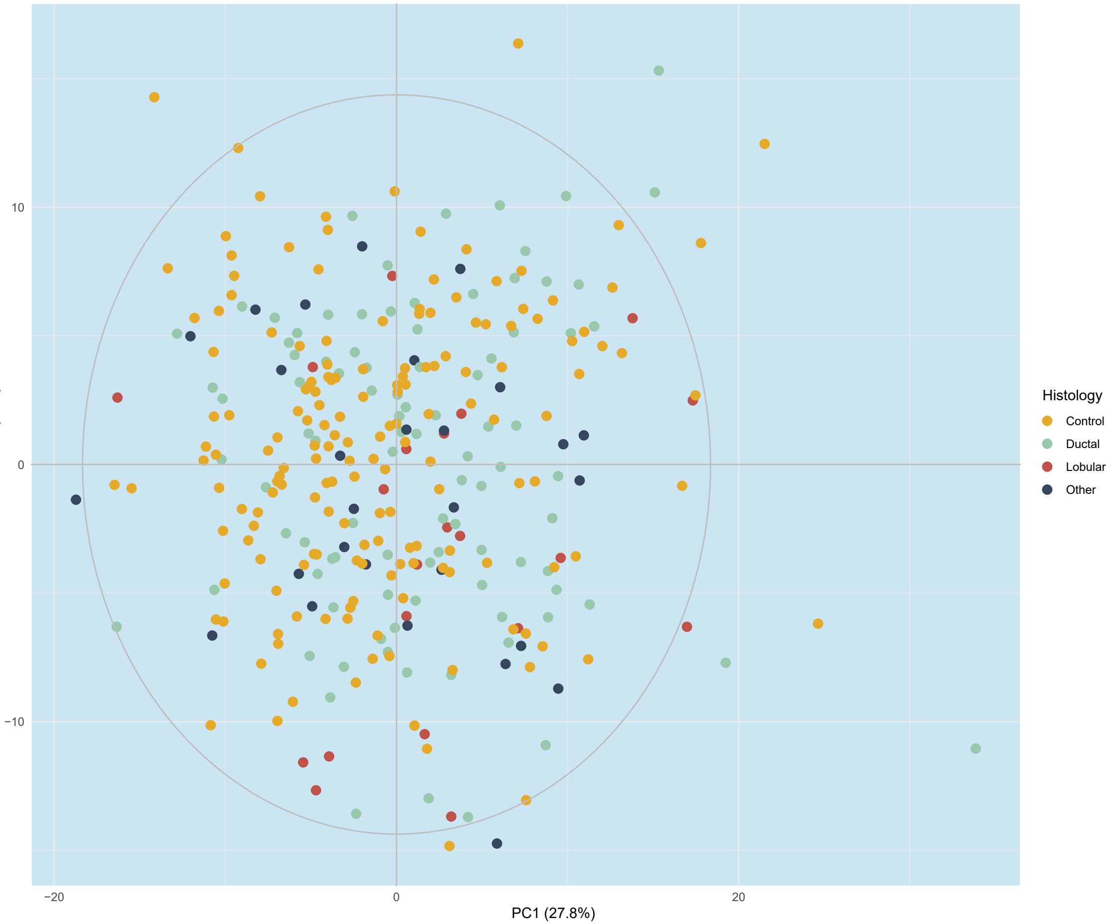
Scores plot
