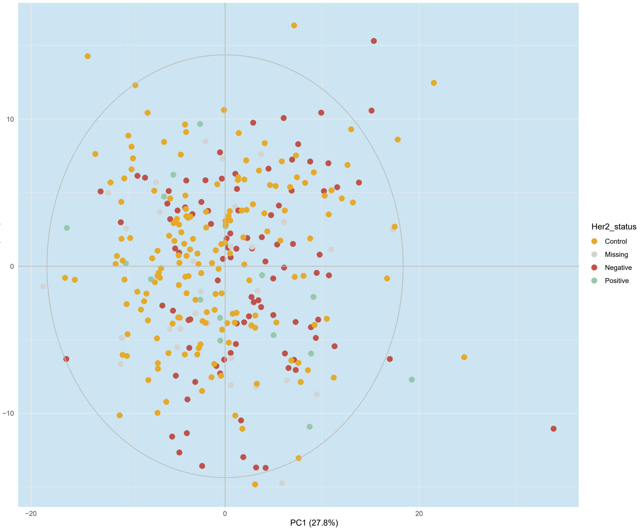
Scores plot
