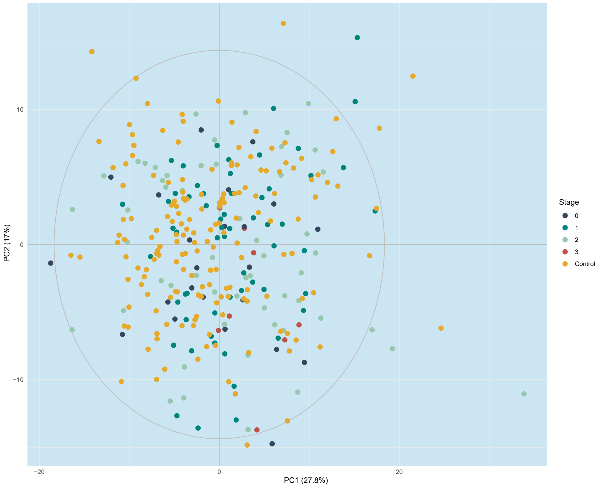
Scores plot
