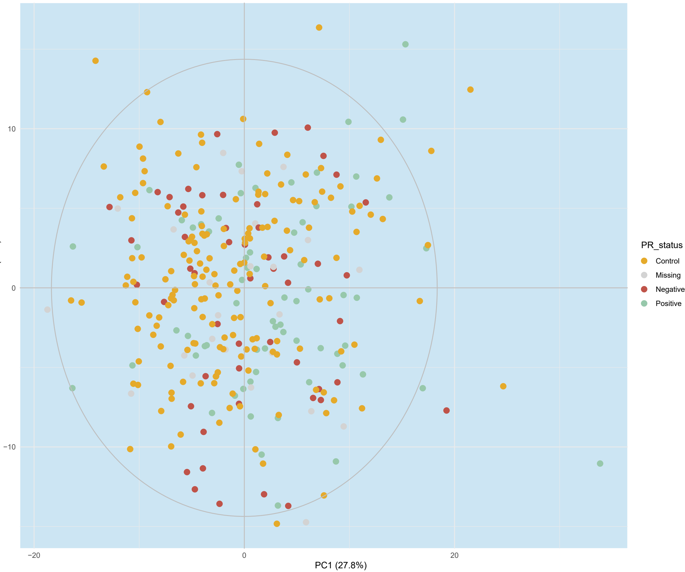
Scores plot
