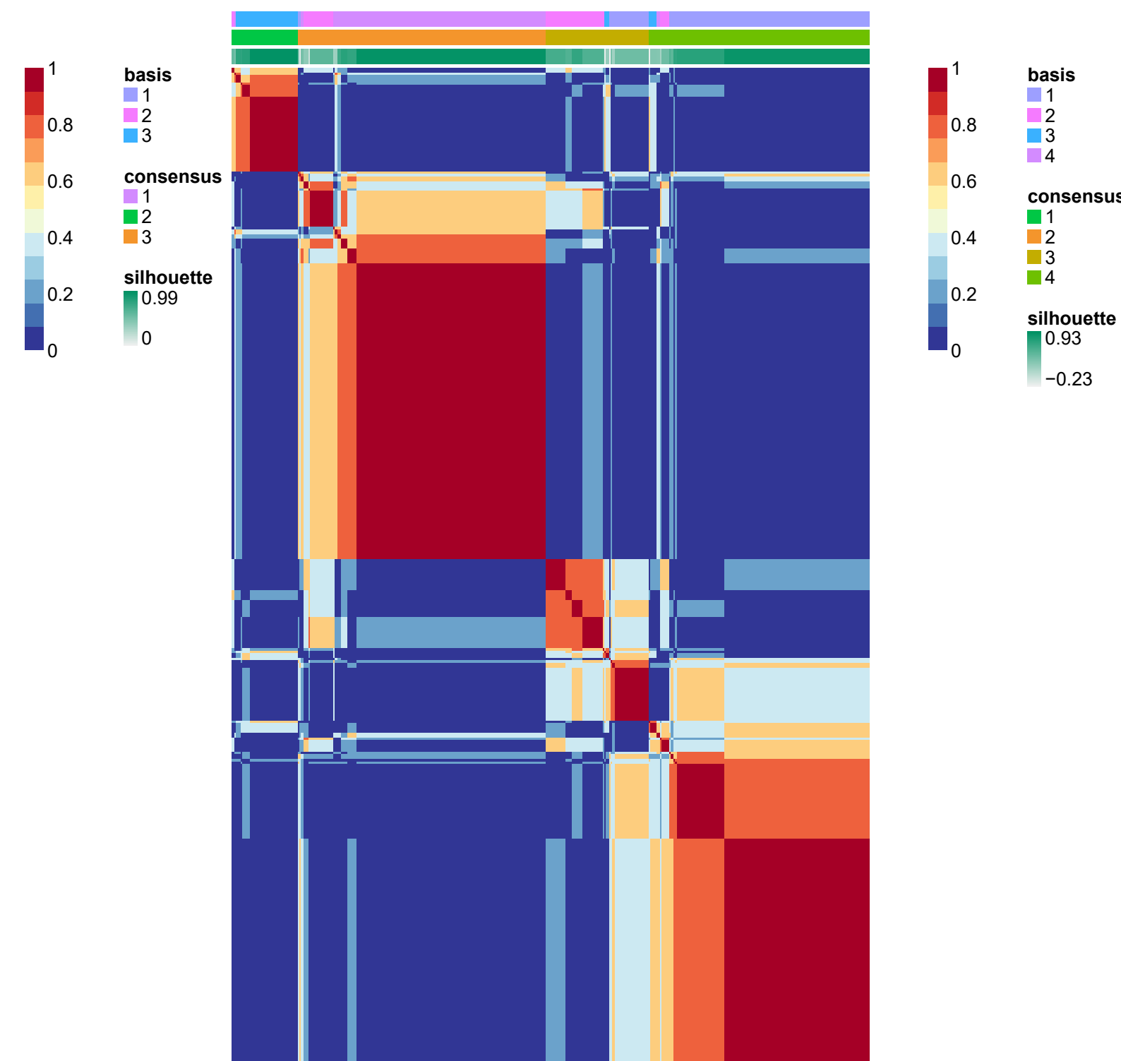
rank = 4
