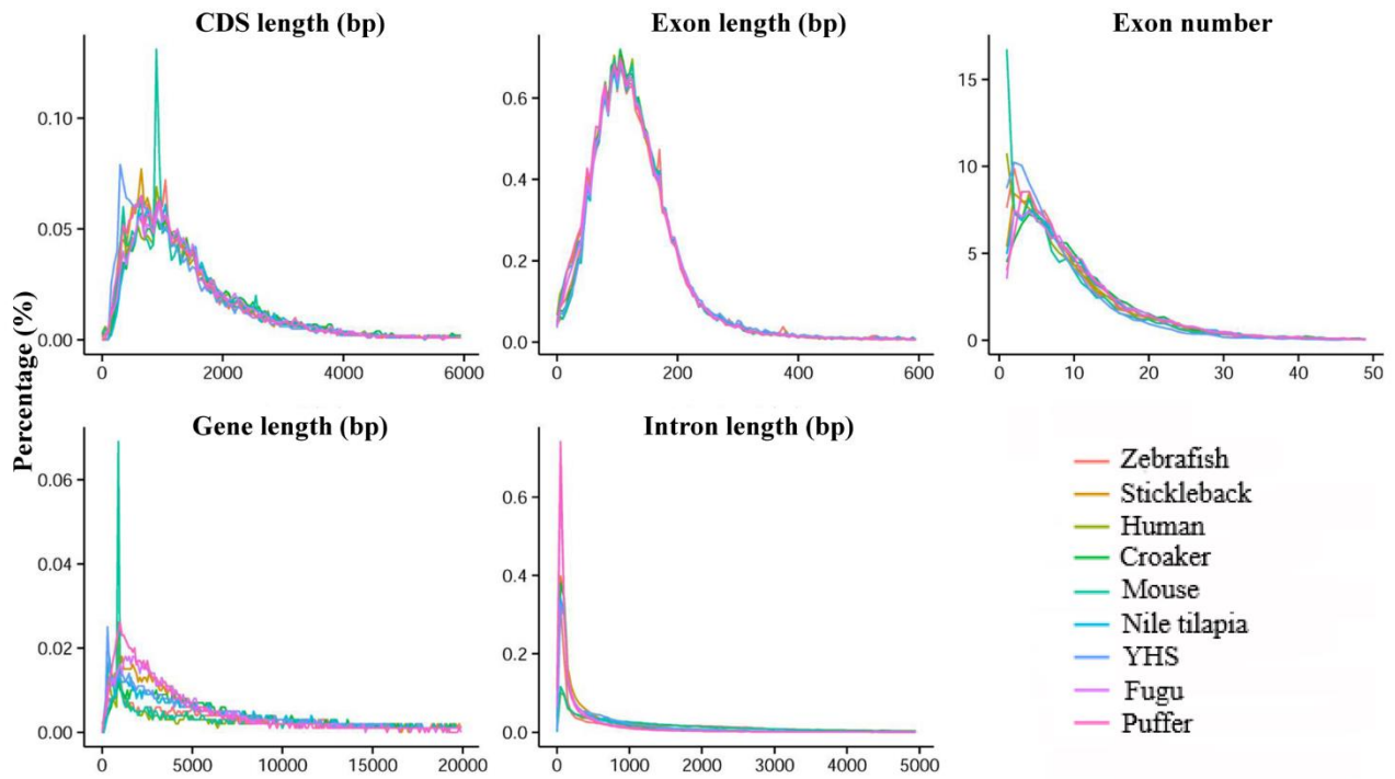
S3 Fig. Comparison of gene structure characteristics among Yap hadal snailfish (YHS) and other vertebrates. The lines with different colors represent different species.
