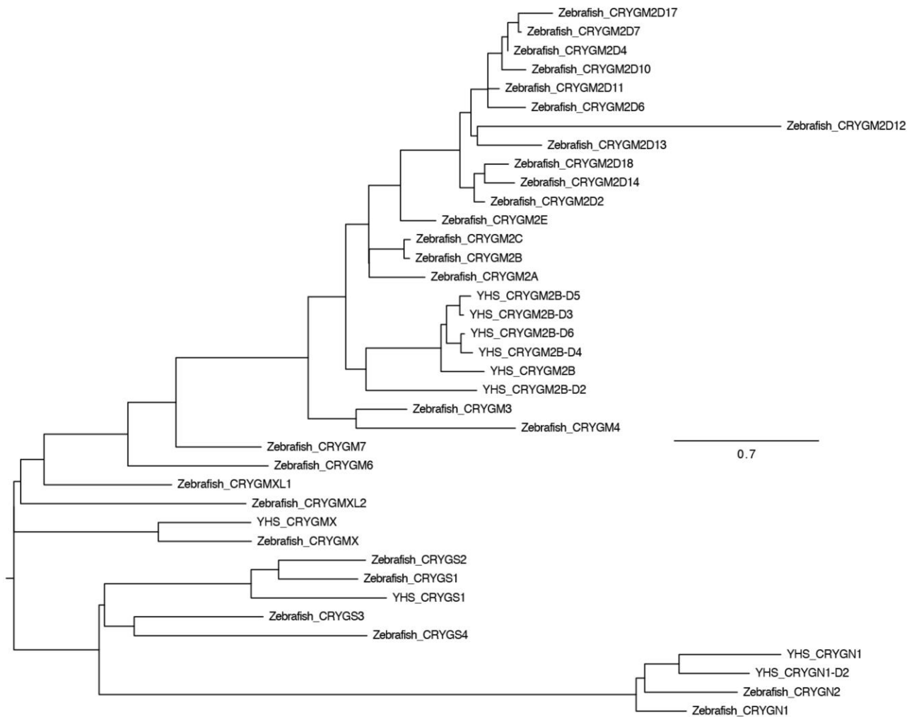
S8 Fig. Phylogenetic tree of the \gamma -crystallin genes of Yap hadal snailfish (YHS) and zebrafish.
