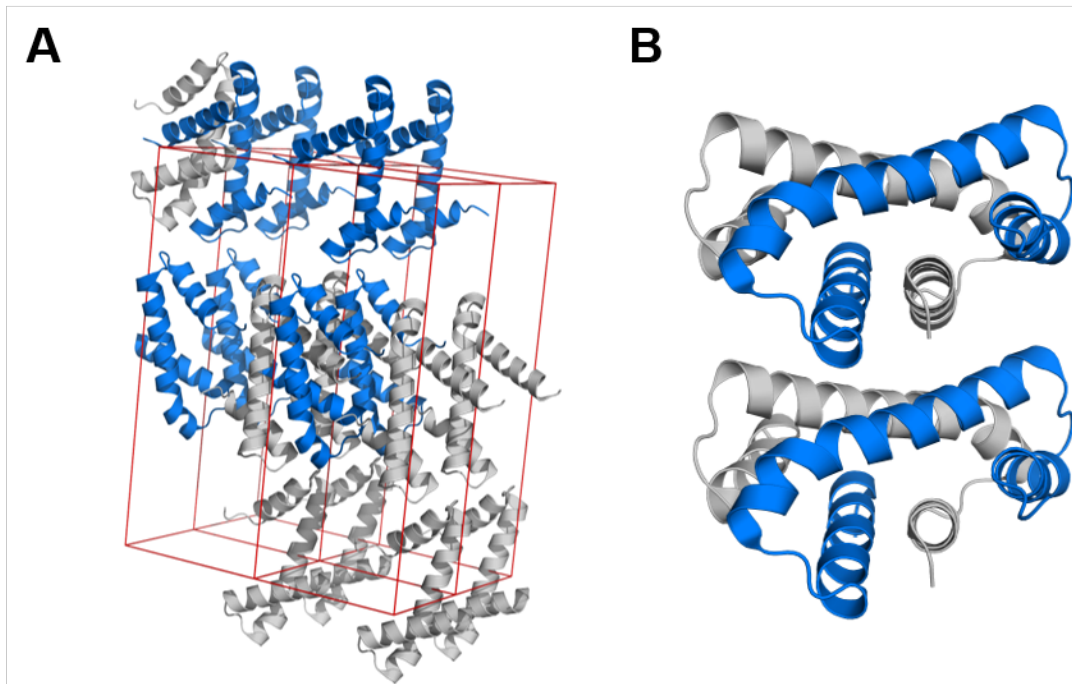
S1 Fig. Crystal packing in dArc2-NL. (A) The unit cell. (B) Stacking of dArc2-NL domain-swapped dimers in the lattice.
