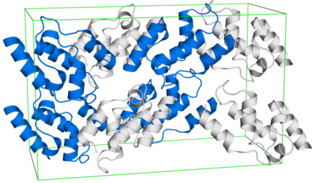
S2 Fig. Crystal packing in dArc1-CL. (A) The unit cell. (B) A monomer of dArc1-CL.
