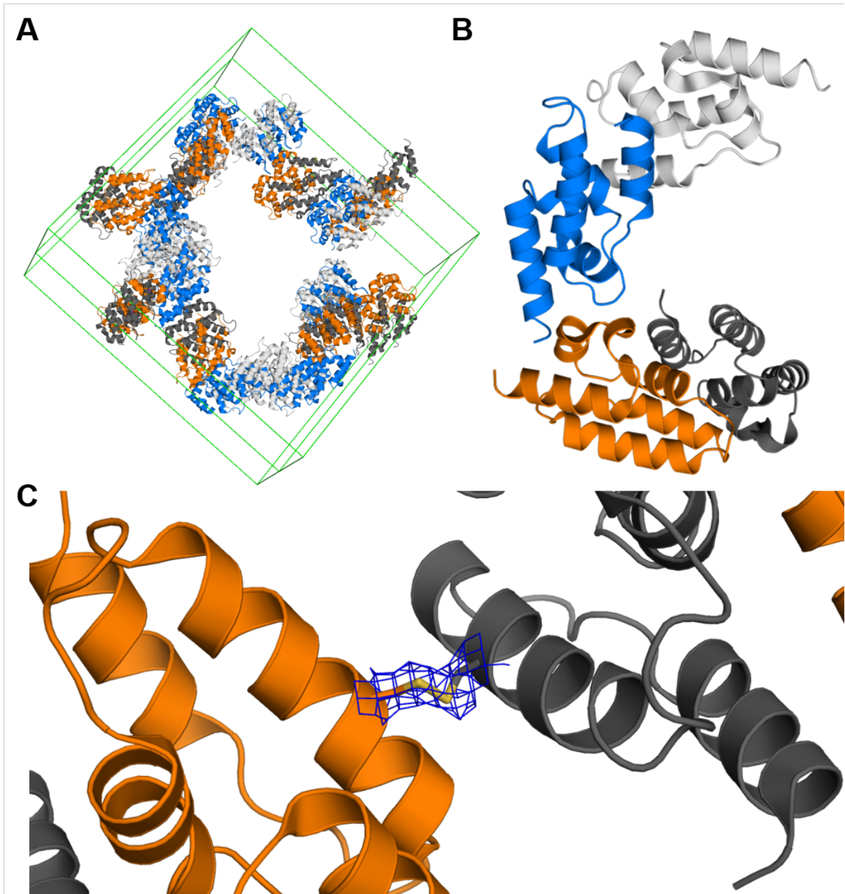
S3 Fig. Crystal packing in dArc2-CL. (A) The unit cell. (B) dArc2-CL is packed as homodimers. (C) In the crystal lattice, dimers are linked to each other via a disulfide bridge.
