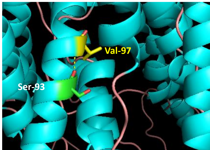
SLC26A4 p.Val97
