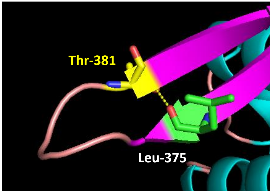
MYO7A p.Thr381Met
