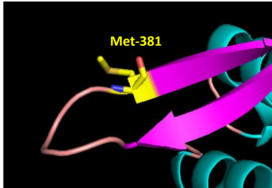
MYO7A p.Thr381Met
