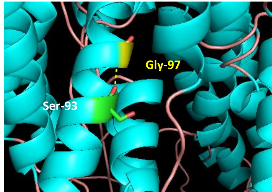
SLC26A4 p.Val97Gly
