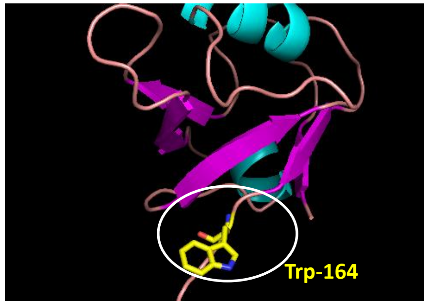
PDZD7 p.Arg164Trp
