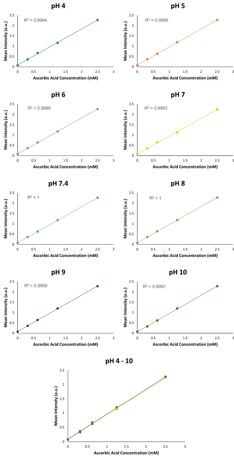
Supplementary Figure 2. The performance of cupric ion-based total antioxidant capacity (CuTAC) assay under different pH level from pH4 to pH10. The CuTAC assay showed highly linear relationship with serial ascorbic acid concentrations under different pH level. The overlapping line charts was illustrated at the bottom of the figure.
