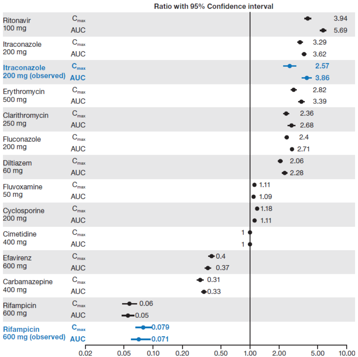
Figure S4. Observed and simulated zanubrutinib geometric mean C_{max} and AUC ratios (95% CI) with various CYP3A4 inhibitors and inducers
