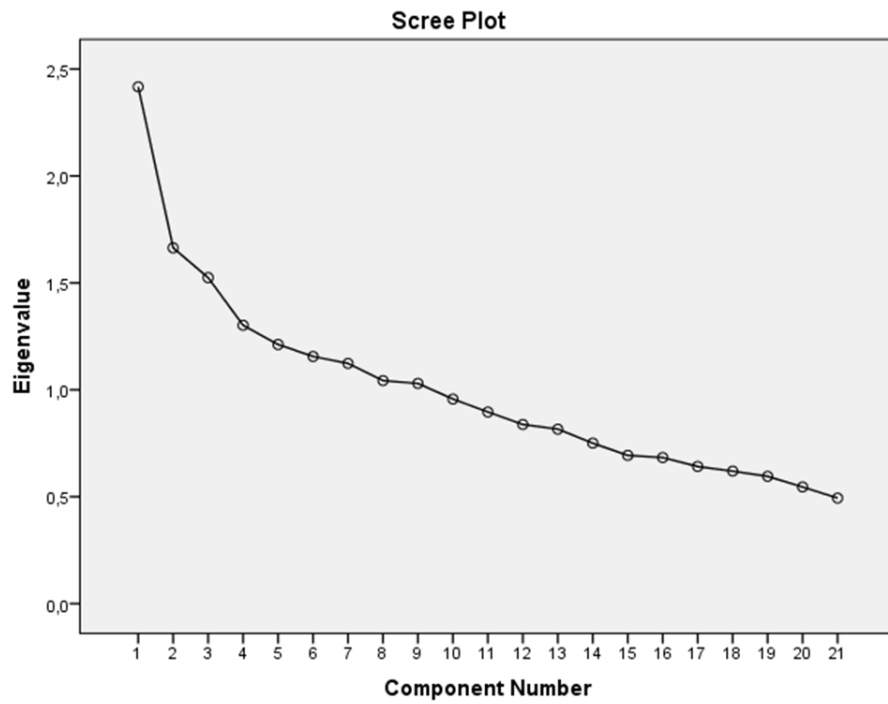
Supplementary figure 1. Scree plot from Principal Component Analysis (n=861)
