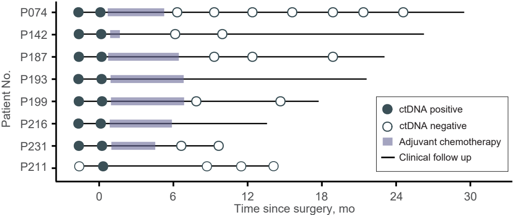
Figure S4. The clinical courses together with ctDNA statuses of 8 out of 20 ctDNA-positive (at day 3-7 post-operation) patients without documented recurrence.
