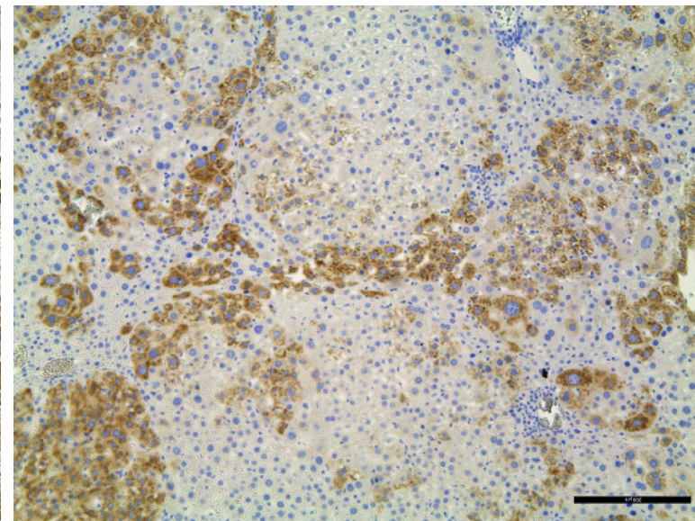
p-mTOR-Ser2448 (100X)
