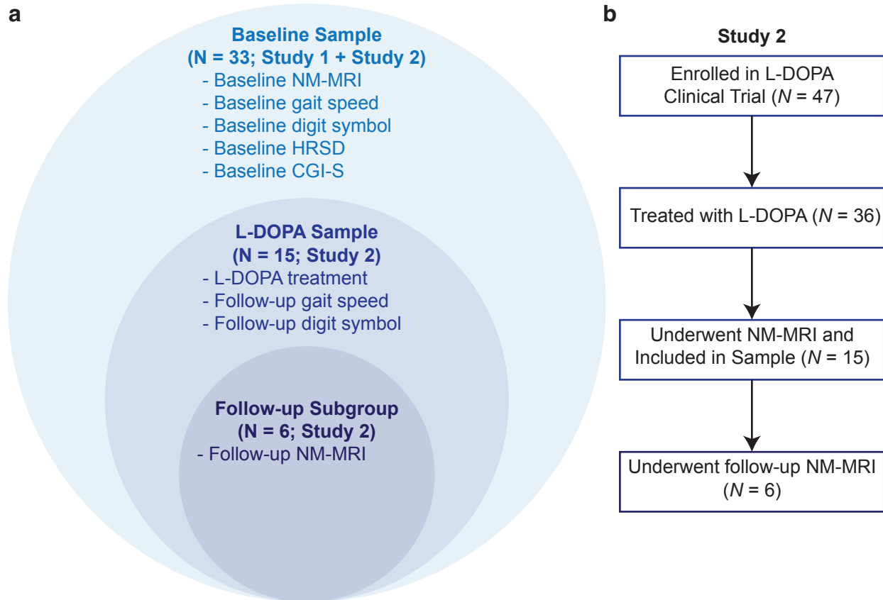
Figure S1. Description of study samples. (a) Venn diagram showing the different samples analyzed in the current study. (b) Flowchart showing the details of subjects from Study 2. We refer the reader to Rutherford et al., Biological psychiatry . 2019;86(3):221-9 for full CONSORT flow diagram.
